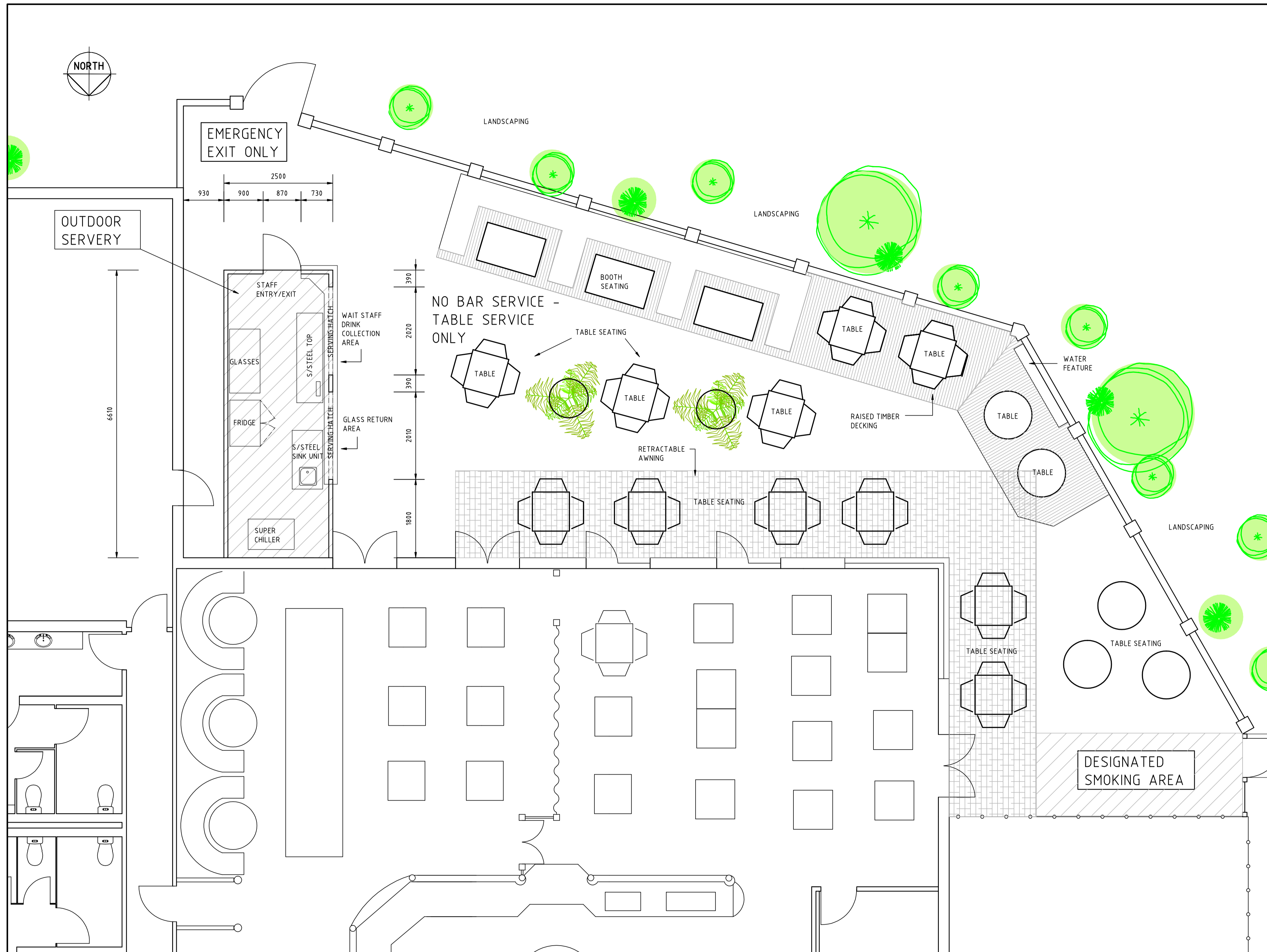
FLOOR PLAN 1:50
